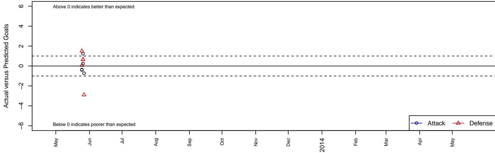
Capital Athletic SA Boca Bravehearts G01 Dots are actual minus expected GF (blue circles) and GA (red triangles). Blue line is smoothed change in attack strength. Red is smoothed change in defense strength.
